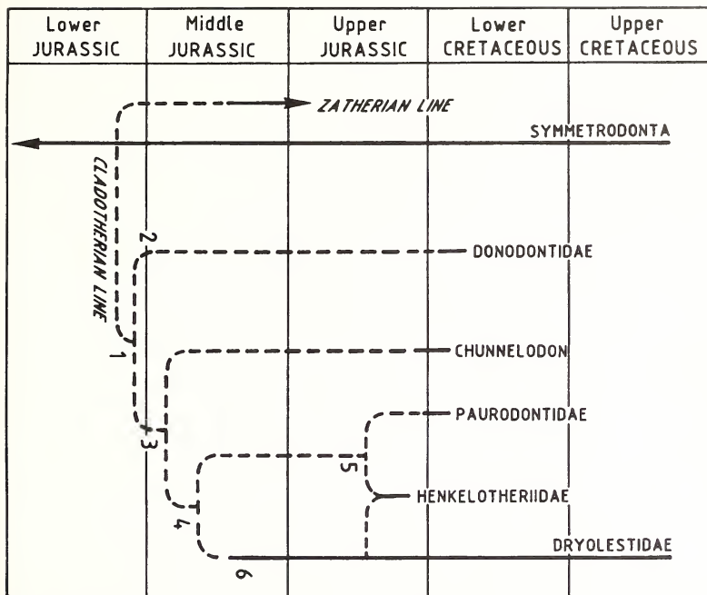
TEXT-FIG. 15. Proposed relationships of the various cladotherian families considered in this paper, based on lower molars only. 1. loss of lingual cingulum on molars; trigonid angle < 100^\circ ; expanded talonid; transverse shear. 2. antero-posterior compression. 3. loss of symmetry; paraconid decreases; loss of anterior cusplule; slightly unequal roots. 4. shelf-like paraconid; procumbent paraconid. 5. decrease in number of molars; paraconid low relative to protoconid. 6. increase in number of molars; antero-posterior compression; strongly asymmetrical roots; talonid decreases.
